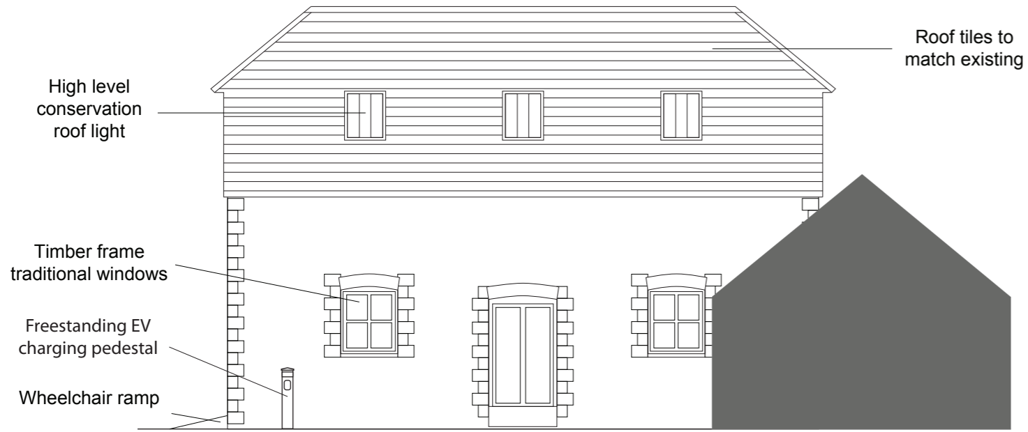
NW Elevation
